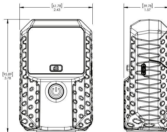
CAL1200 Dimensions
