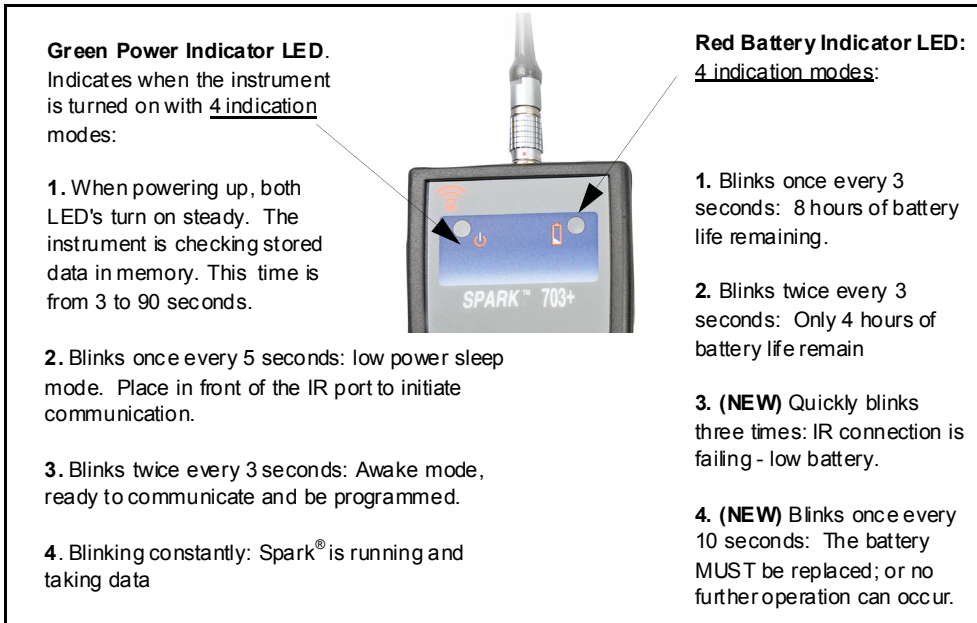
FIGURE 1-16 Indicators on Front Panel of 703+ and 705+ instruments
